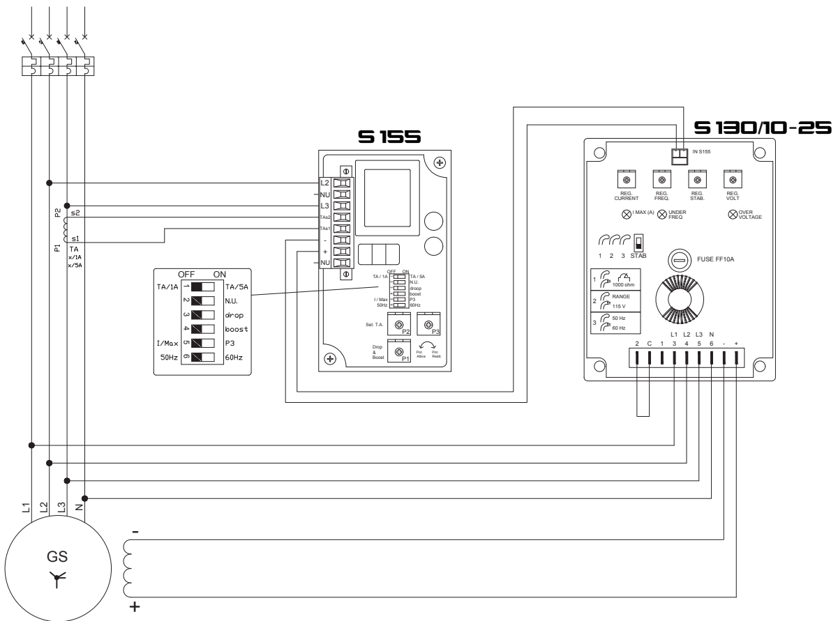
PIC.1 - Connecting diagram between an S155 Reactive Power Sharer and a S130/10-25
