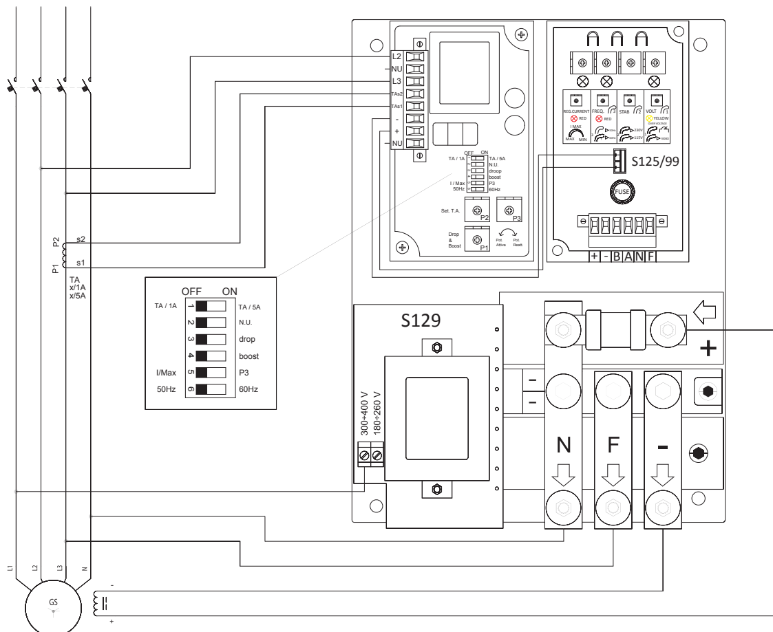
PIC.2 - Connecting diagram between an S155 Reactive Power Sharer and a S099 AVR
